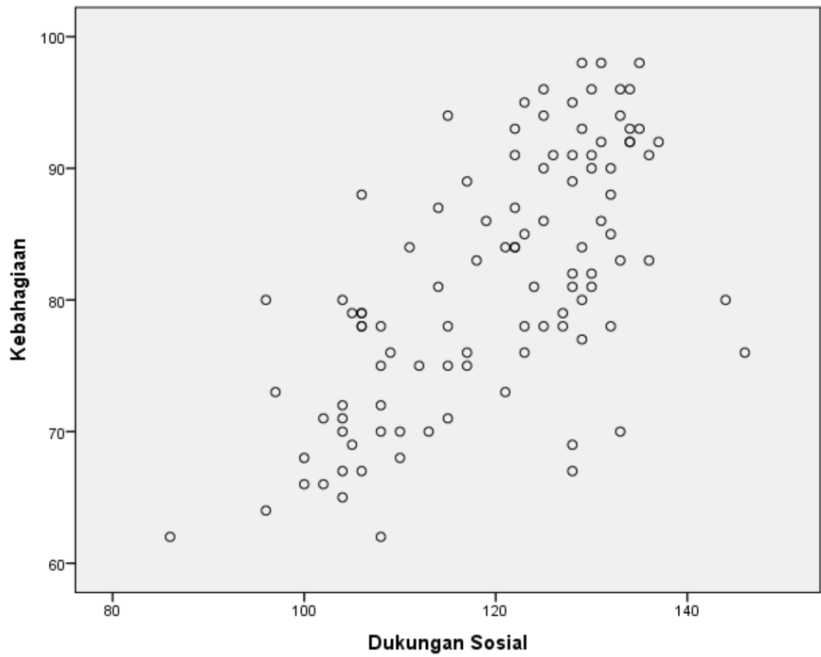
Scater Plot
