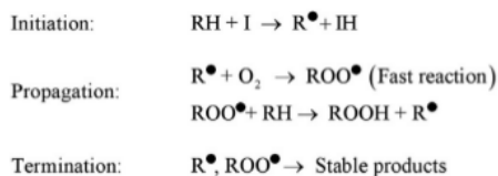
Fig. 1. Primary oxidation reaction mechanism.
