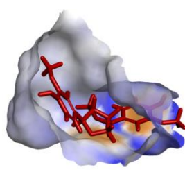
(-)-pinoresinol
