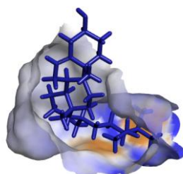
Beta sitosterol
