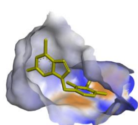
Native ligand 3QDD
