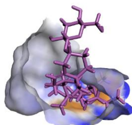
Daucosterol
