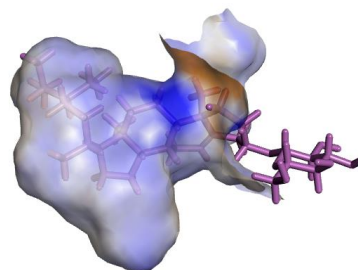
Daucosterol
