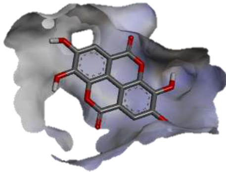
Ellagic Acid
