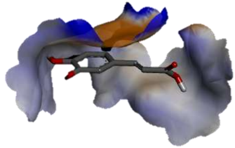
Ferullic Acid
