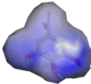
Gallic Acid
