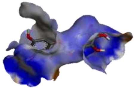
Myricetin
