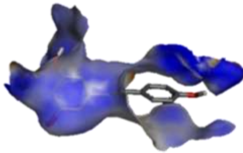
Resveratrol
