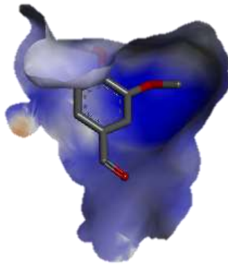
Vanillin
