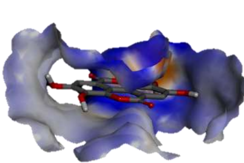
Ellagic Acid
